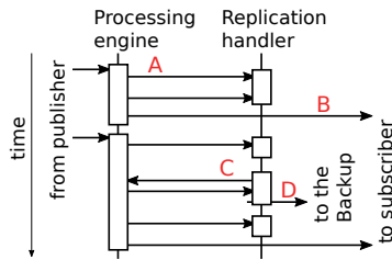
Fig. 5. Interactions between ARREC components.
