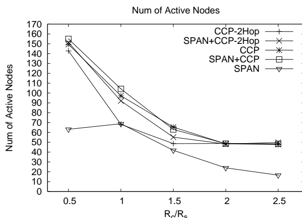
Fig. 22. Number of active nodes vs. R_c/R_s . The protocols that integrate CCP result in more active nodes in order to achieve coverage. Two-hop protocols result in fewer active nodes than their one-hop counterparts due to the knowledge of more active nodes within sensing neighborhood.
