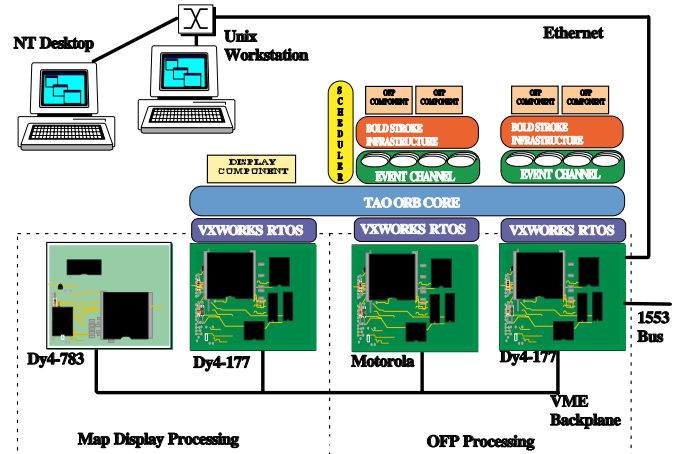
Figure 1: Open Experimentation Platform Hardware and Software
