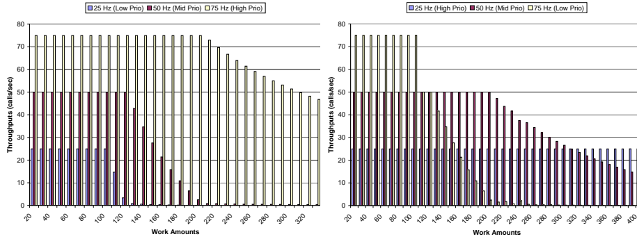
Fig. 8. IRIP with Threadpool Lanes Fig. 9. IRDP with Threadpool Lanes
