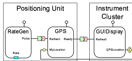
Fig. 4. CIAO Example Design
