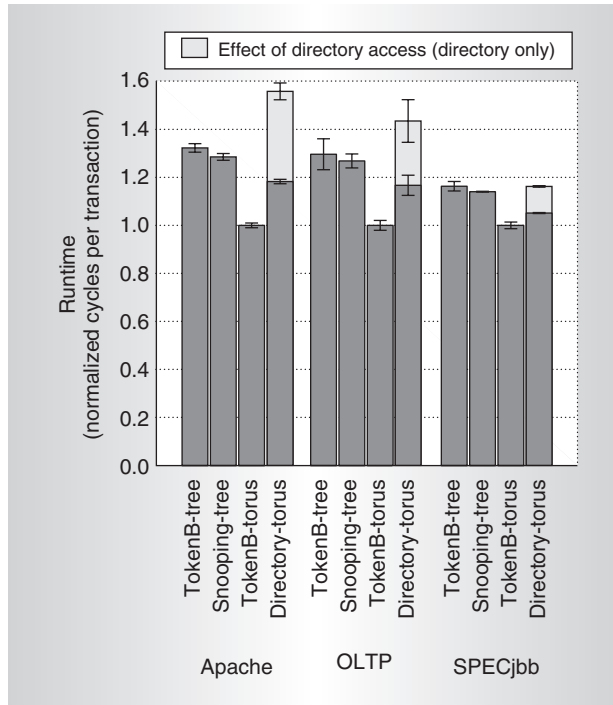
Figure 4. Runtime normalized to TokenB on the torus interconnect.
