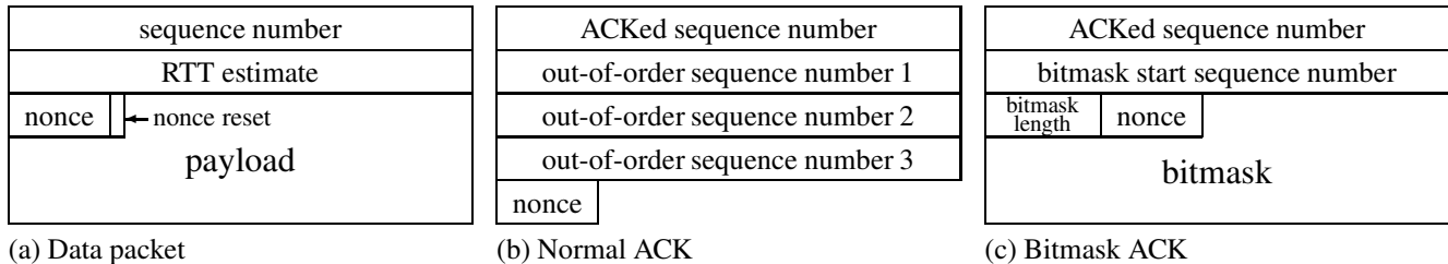
Figure 3. Packet header formats in RTFRC
