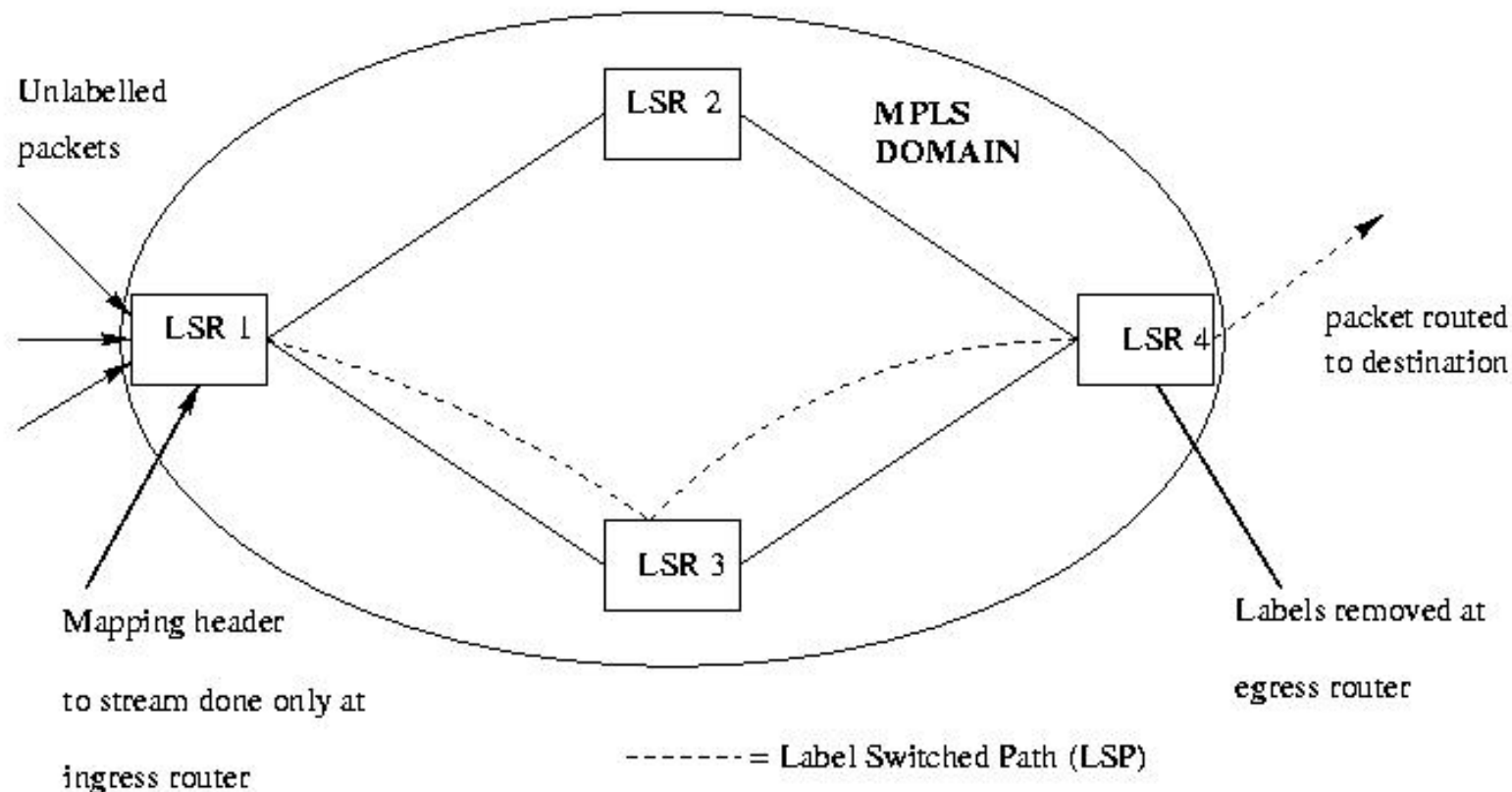
Figure 7: The MPLS Architecture
