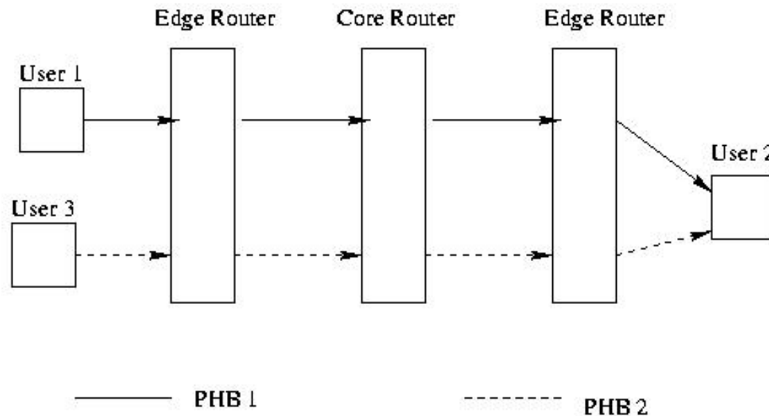
Figure 5 : The DiffServ Architecture
