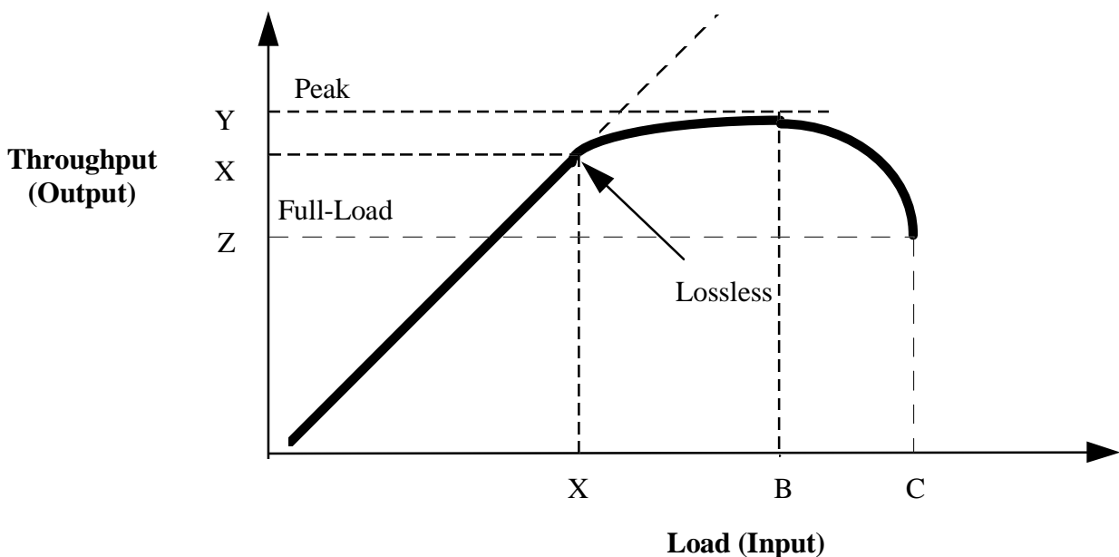
Figure 3.1: Peak, lossless and full-load throughput
