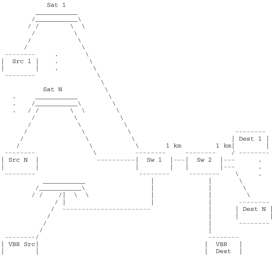
Figure 5: The "N Source + VBR" Configuration with long feedback delays
