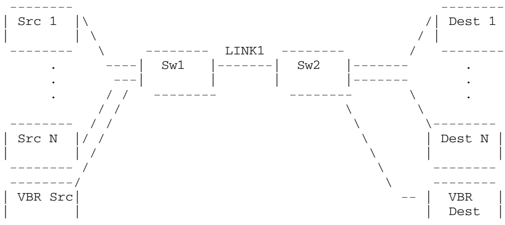
Figure 3: The "N Source + VBR" Configuration
