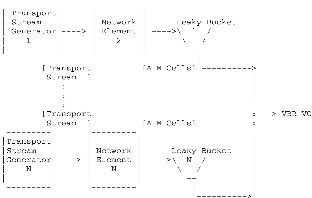
Figure 2: Multiplexing MPEG-2 Compressed Video Traffic over VBR
