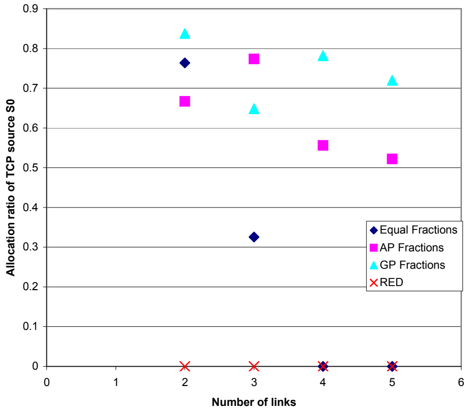
Figure 13 - Allocation Ratio of TCP Flow-0 in MCL for LEO satellite networks
