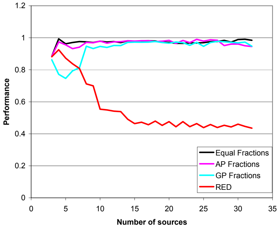
Figure10- Performance in SCL with TCP and UDP flows for GEO satellite networks
