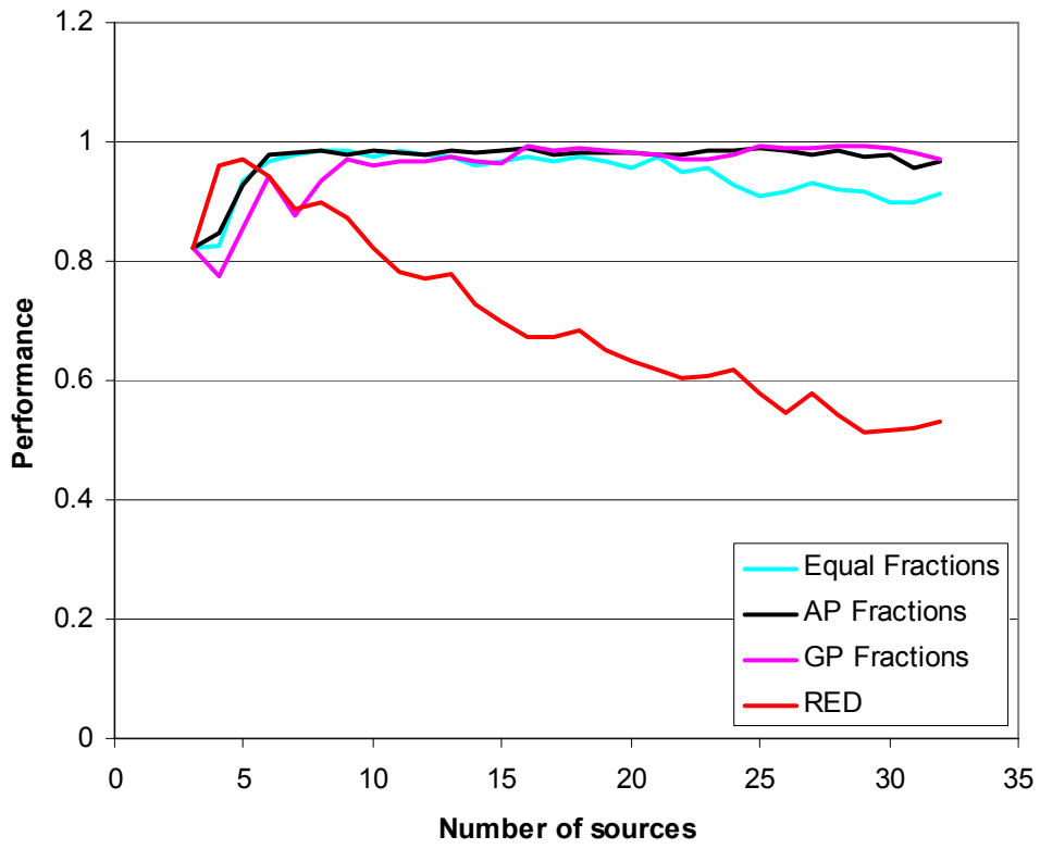
Figure 9- Performance in SCL with TCP flows in GEO satellite networks
