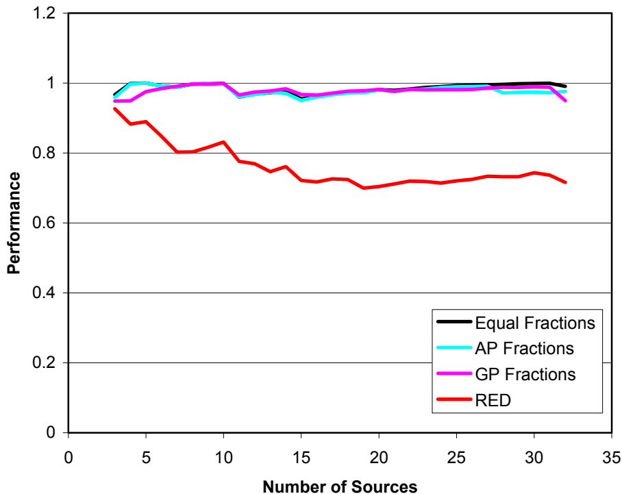
Figure 8- Performance in SCL with UDP flows in GEO satellite networks
