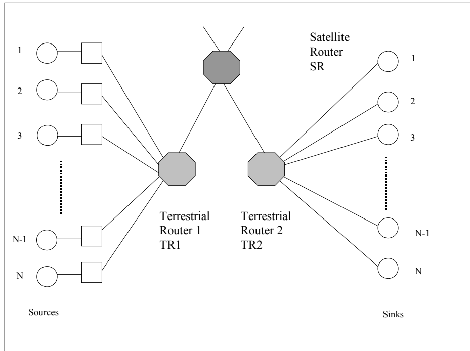
Figure 7 - Single Congested Link in Satellite Network - Network Configuration
