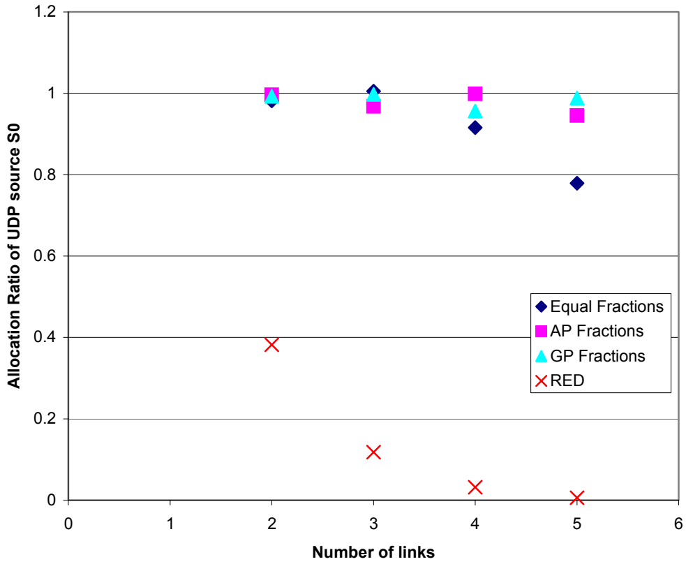
Figure 12 - Allocation Ratio of UDP Flow-0 in MCL for LEO satellite networks
