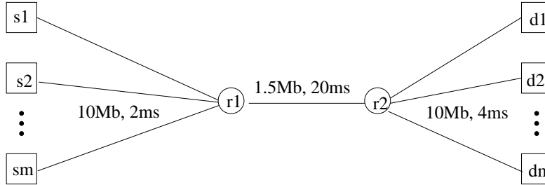
Figure 2: Simulation model.
