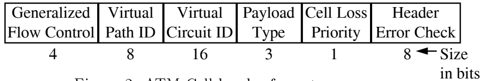
Figure 2: ATM Cell header format
