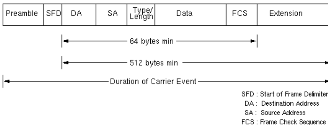
Fig 1. Ethernet Frame Format with Carrier Extension
