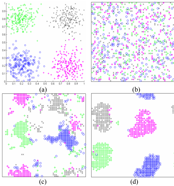
Figure 1. The process of clustering of A^4C . (a) Data distribution in the attribute space (b) Initial agent distribution in the grid (c) Agents' distribution after 10000 iterations (d) Agents' distribution after 20000 iterations
